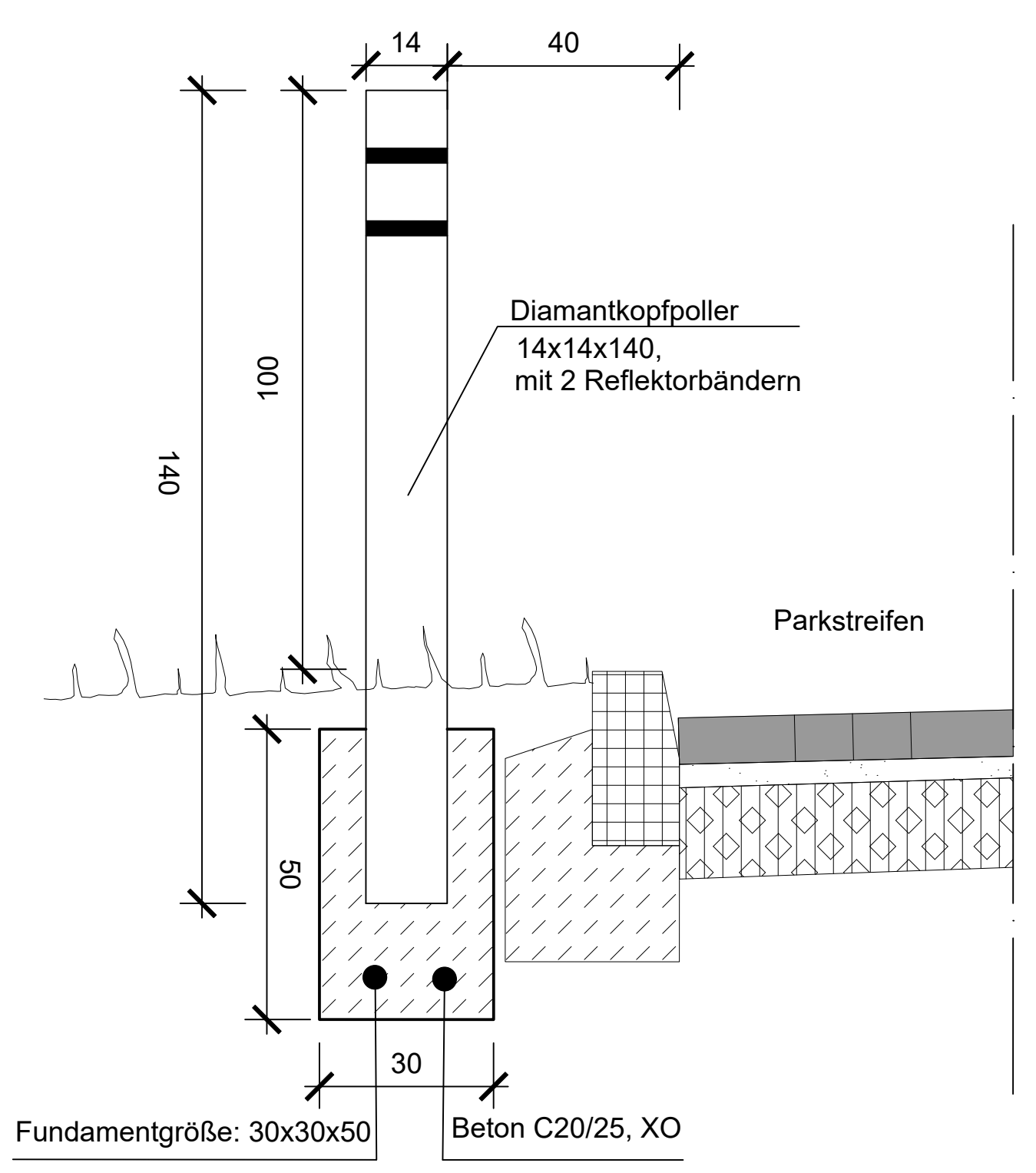
Detail Diamantkopfpoller
